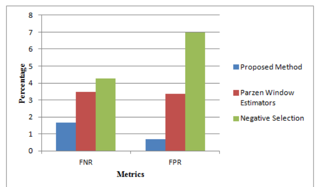
Fig. 3. Performance analysis of various schemes based on FNR and FPR for Dataset 1.
