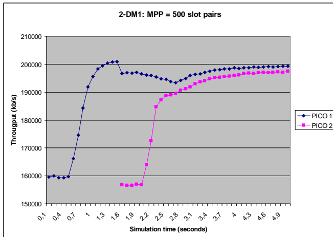
Fig.6. Scenario 2: Throughput for 2-DM1 packet and MPP = 500
