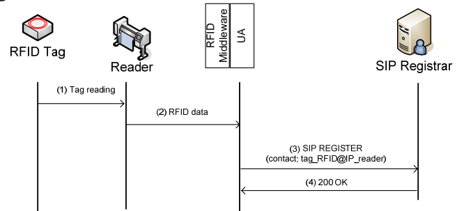
Fig. 6 – Registration procedure
