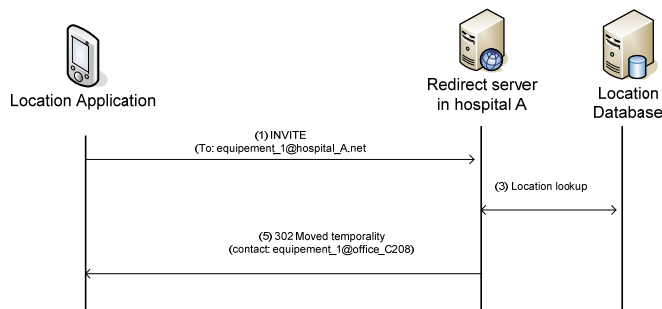
Fig. 7 – Tracking procedure
