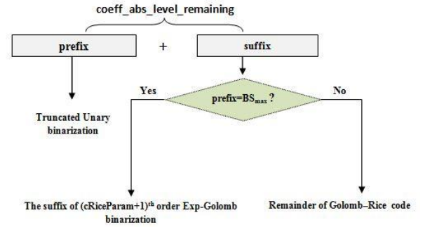
Fig. 2. Binarization of coeff_abs_level_remaining : prefix is binarized with truncated unary code, and suffix is binarized either by Golomb-Rice code or by Exp-Golomb code
